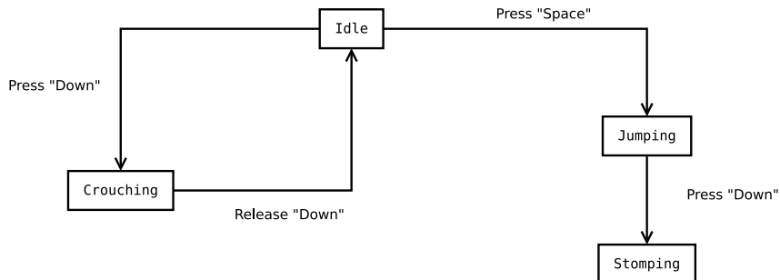
Figure 322: Diagram of a character’s state machine
